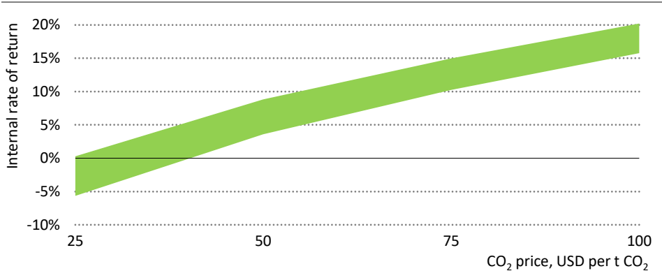
Figure 4.21 ▶ Rate of return for a coal CCUS retrofit project in China earning revenue solely by selling CO 2 certificates
