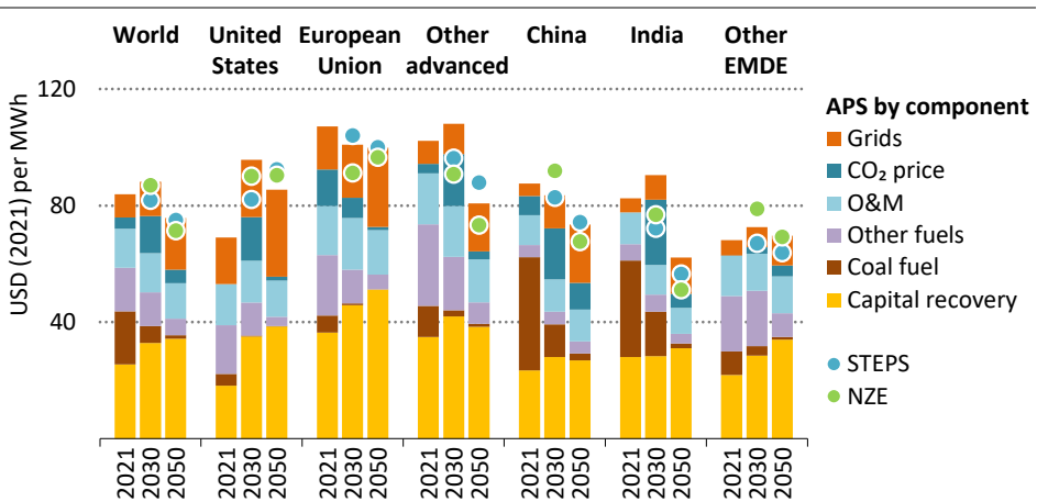
Figure 2.19 ▶ Electricity system costs per unit by component, region and scenario, 2021-2050
