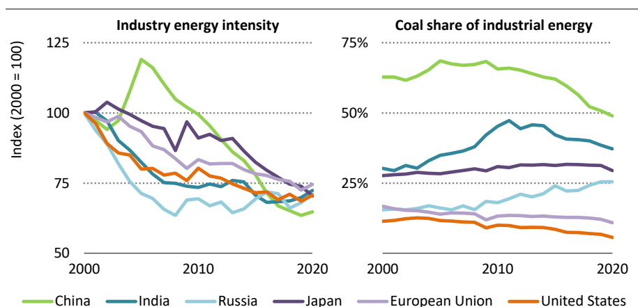
Figure 3.10 ▶ Energy intensity of industry and coal share of industrial energy consumption by region, 2000-2020
