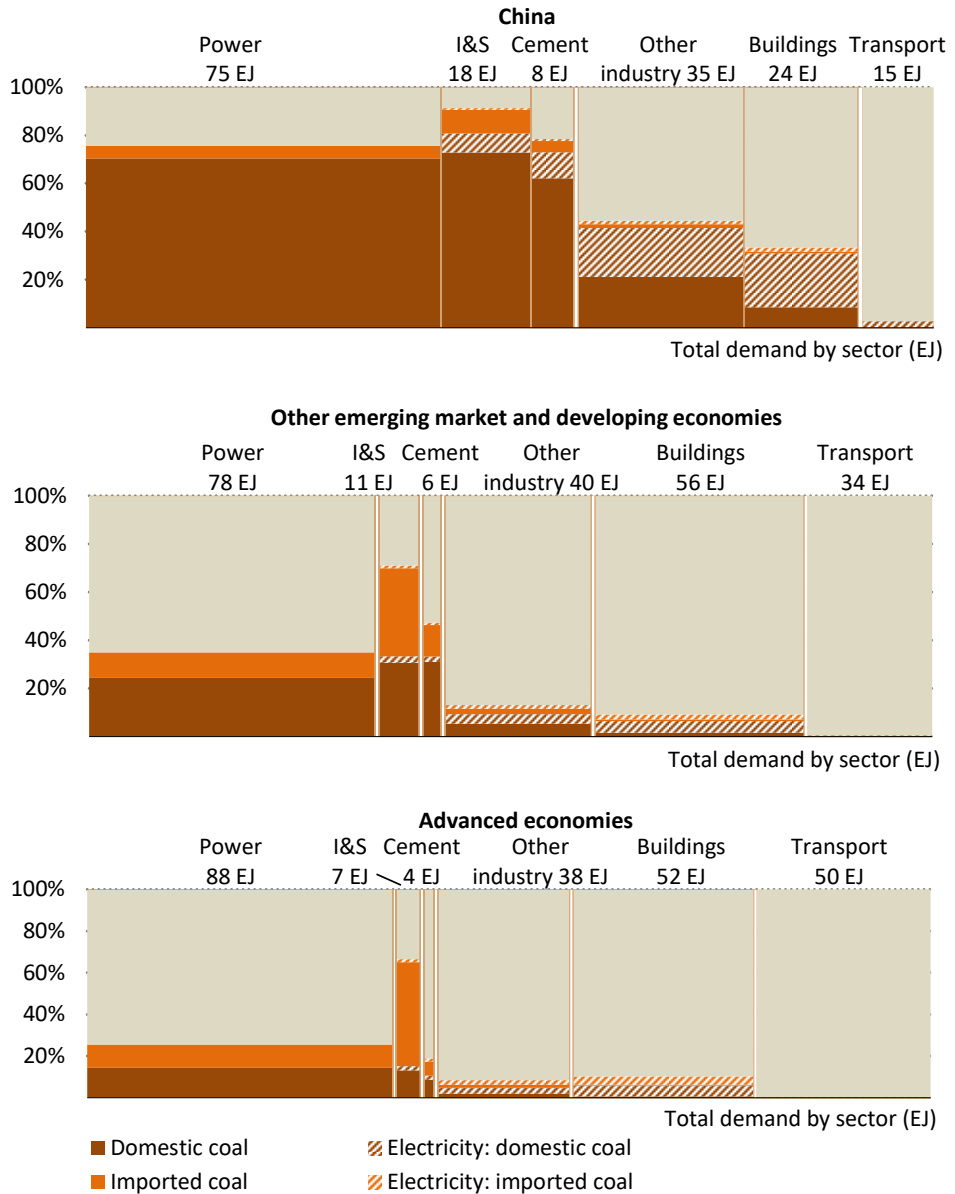
Figure 1.2 ▶ Domestic and imported coal demand by sector and region, 2021
